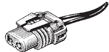
400482 12101898, PT168 Repair Harness - Headlamp Socket For #9005 Halogen Bulb (High Beam) 2 Prong, Two Indexing Grooves 2 - 10" Leads, 18 Ga. Wire GM '86 - UP, Ford, Chrysler Box Qty. 5
