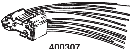
400307 11-18 Ga. (TXL) Leads 8" Length Box Qty. 1
