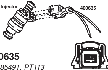
Fuel Injector
